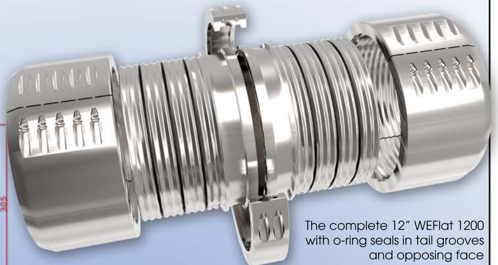
12" WEFlat1200 'quick clamp' joining clamp
